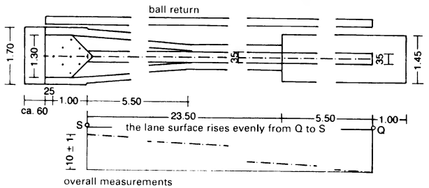
⑤ Alternative skittle alley
